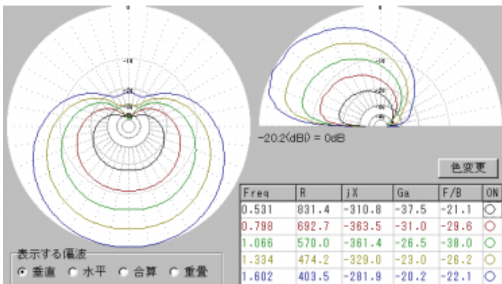
3. H=5m,L=15m,Rt=1000 Ω
