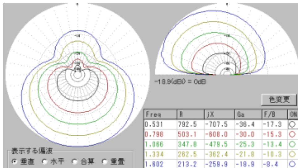
10. H=3m, L=25m, R_t=1580\ \Omega
