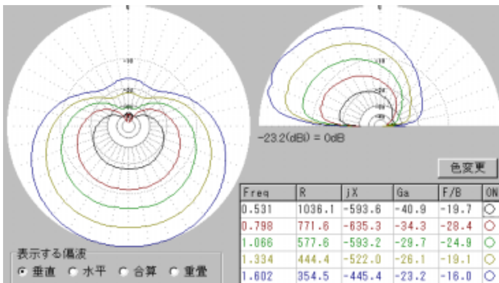
8. H=3m, L=15m, R_t=1440\ \Omega
