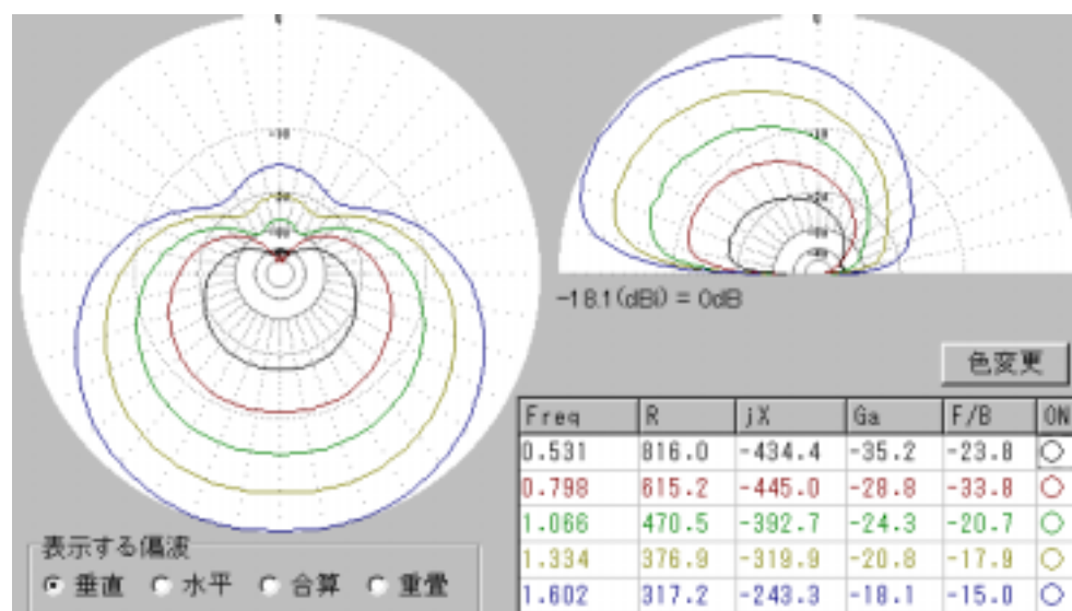
4. H=5m,L=20m,Rt=1140 Ω
