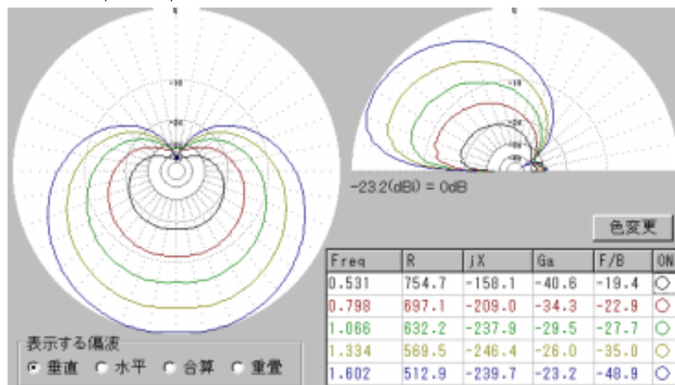
2. H=5m,L=10m,Rt=810 Ω
