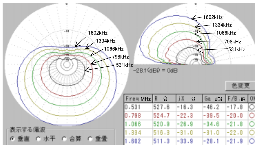
1. H=5m,L=5m,Rt=530 Ω
